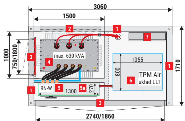
Mzb1 (3,06x1,71) 20/630-3"a"
