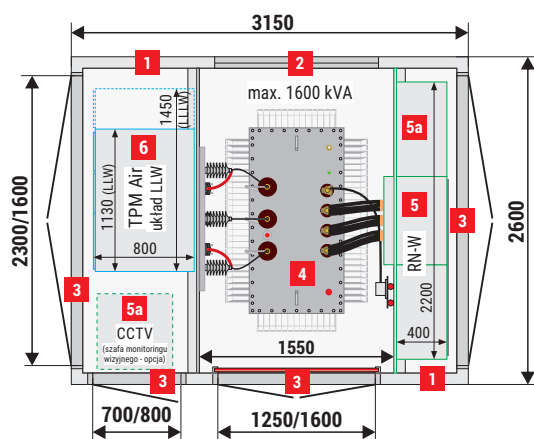
Mzb2 (3,15x2,6) 20/1600-3 (Slave)
