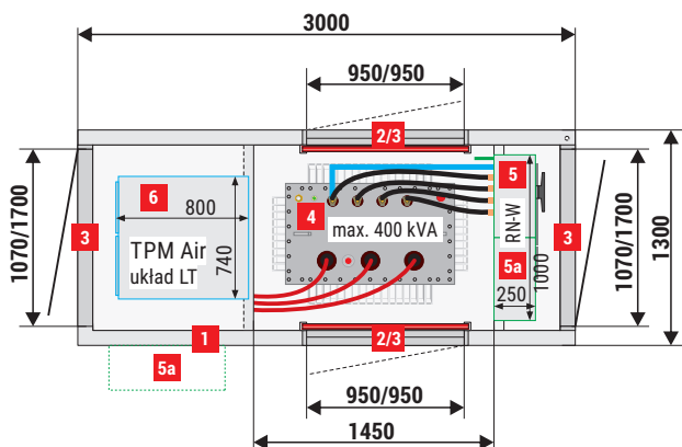
Mzb2 (3x1,3) 20/400-2"a"
