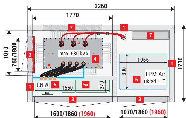
Mzb1 (3,26x1,71) 20/630-3"a"
