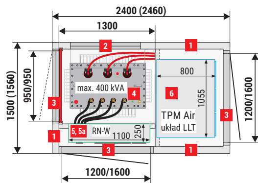
Mzb2 (2,4x1,5) 20/400-3"b"
