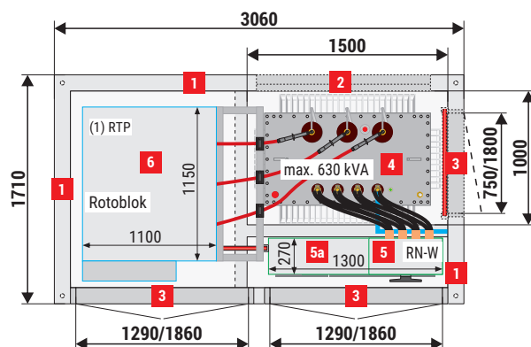
Mzb1 (3,06x1,71) 20/630-1"b"
