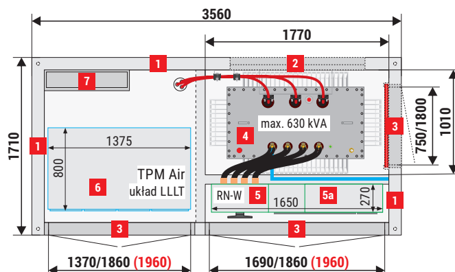
Mzb1 (3,56x1,71) 20/630-4"b"
