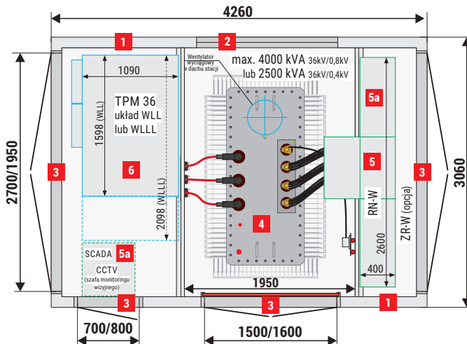
Mzb2 (4,26x3,06) 30/4000-3 (Slave)
