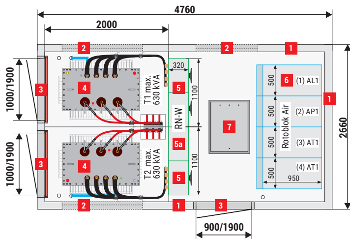
MRw-b(pp) 20/2x630-4"b" wariant II
